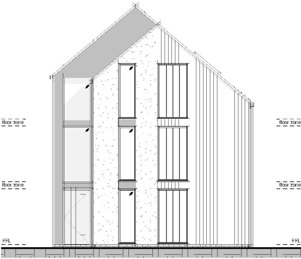
Unit 1 - East (Front) Elevation 1 : 100
