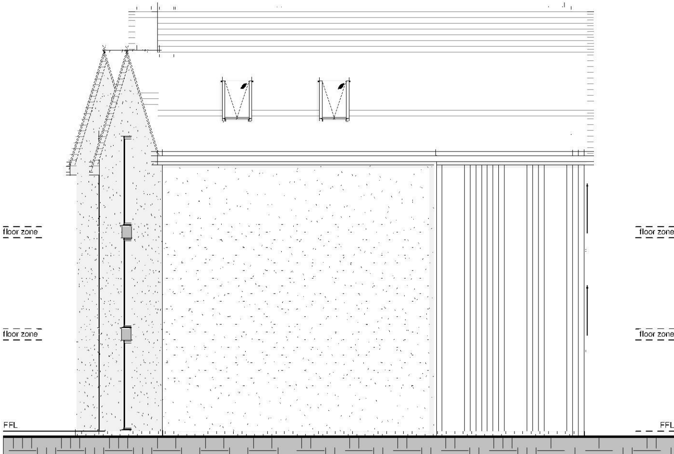
Units 2-4 - North (Side) Elevations 1 : 100
