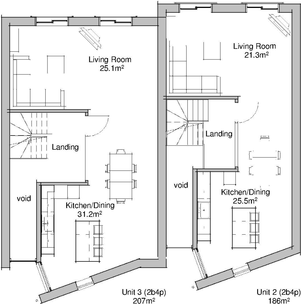
Units 2&3 - First Floor Plan 1 : 100
