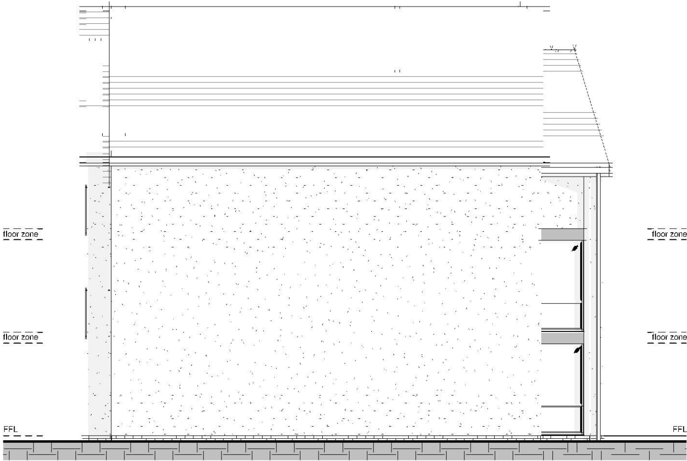
Units 2-4 - South (Side) Elevations 1 : 100
