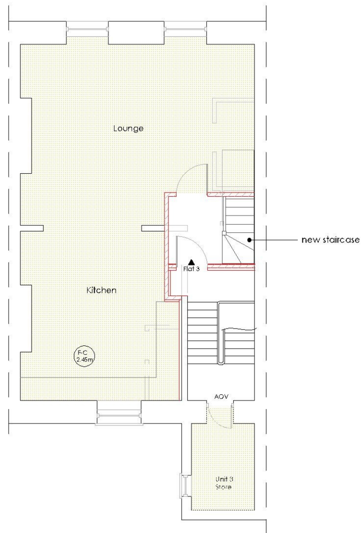
Second Floor Plan - Proposed Unit 3 - 2 person 2 bedroom GIA 84m 2
