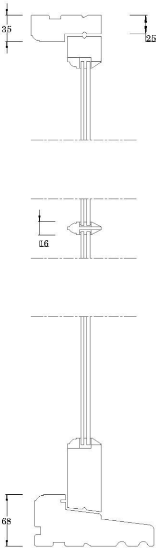
Typical Vertical Section
