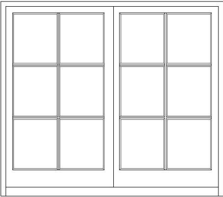
Dormer Bedroom Windows Scale 1:20
