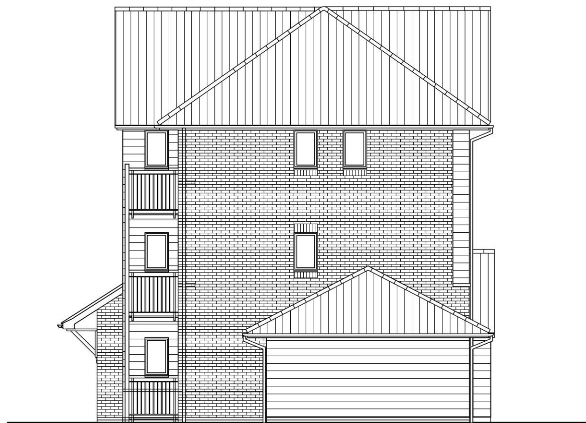
SIDE ELEVATION
