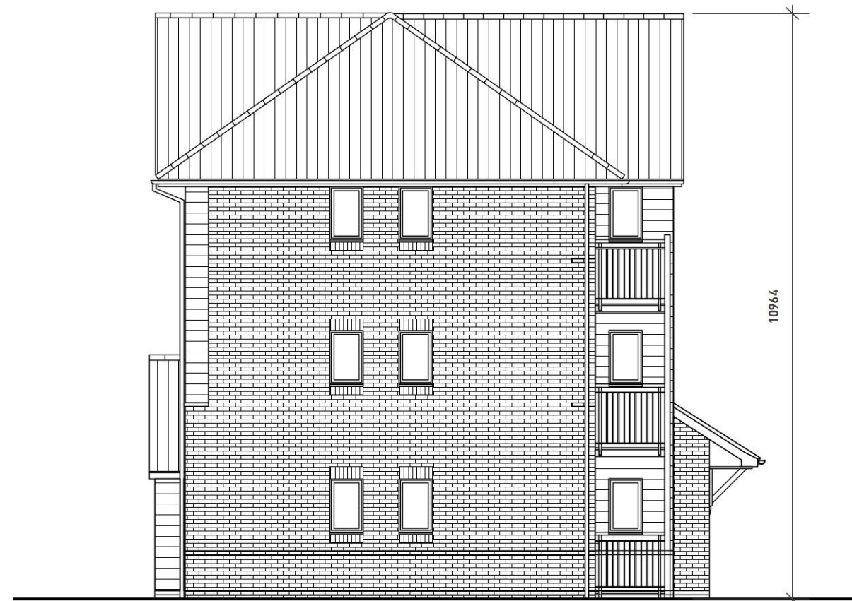
SIDE ELEVATION
