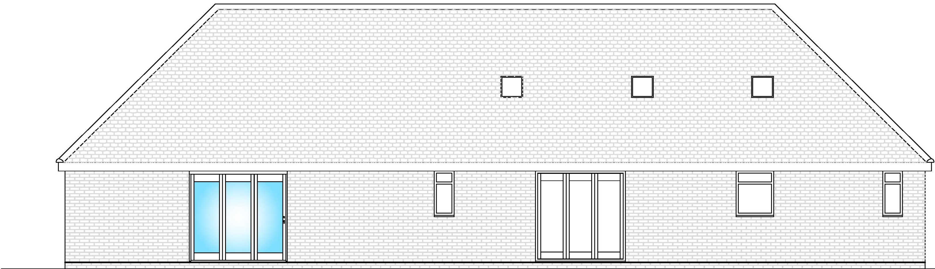
West Elevation
