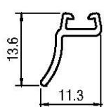
Art. No. 219350 Deep Bottom Rail Front Gasket
