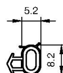
Art. No. 235203 Foamasil Universal Gasket
