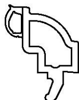
Art. No. 559590 24mm Sculptured Bead Silver Co-Ex
