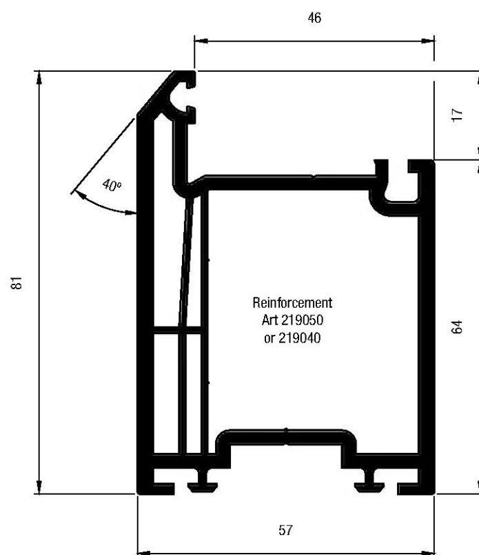
Art. No. 559540 Deep Bottom Rail
