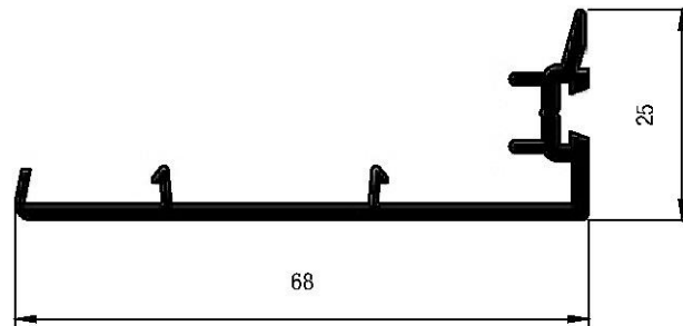
Art. No. 559550 Slim Sash Interlock
