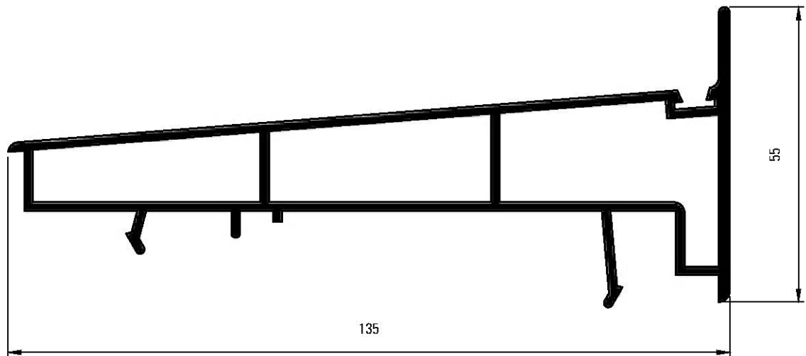
Art. No. 219160 Clip in Sill
