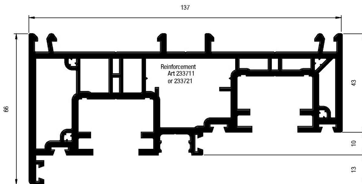
Art. No. 559500 Outer Frame
