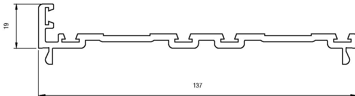
Art. No. 219170 Mullion Adaptor Profile
