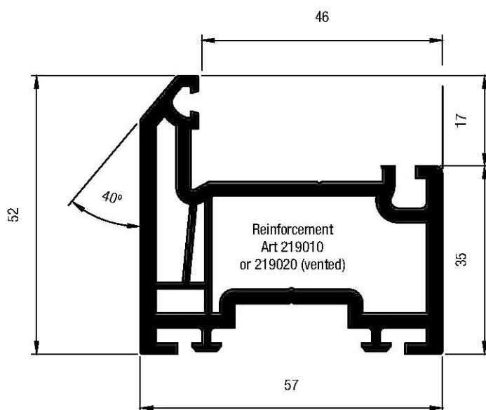
Art. No. 559520 Intermediate Sash
