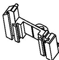
Art. No. 219270 Intermediate Sash Joint Block Scale 1:2
