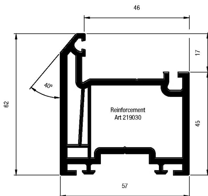
Art. No. 559530 Large Sash
