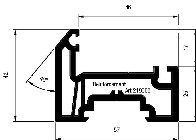
Art. No. 559510 Slim Sash
