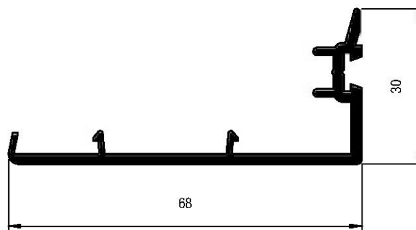
Art. No. 559560 Large Sash Interlock
