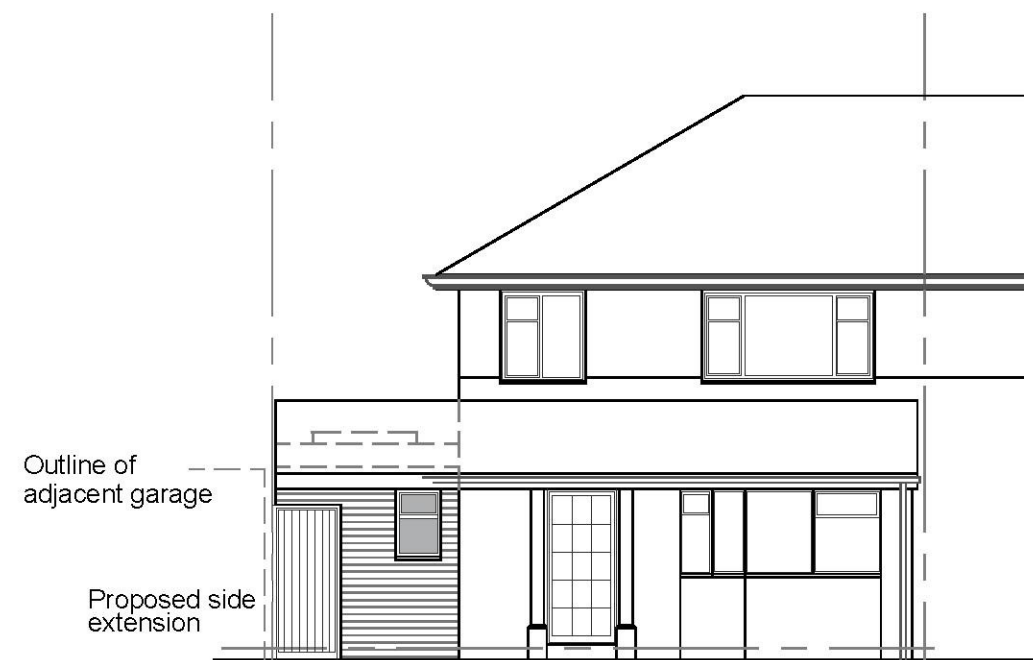
PROPOSED FRONT ELEV
