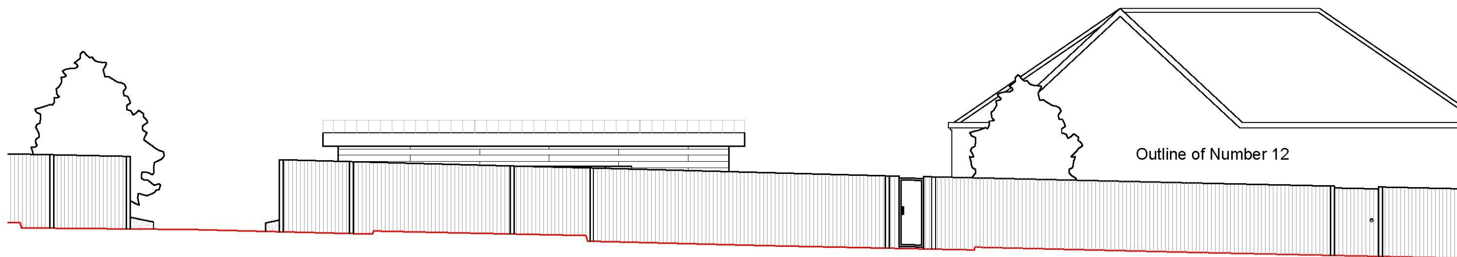
Proposed Street Elevation
