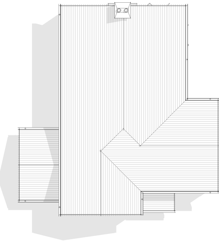
3 Proposed Roof Plan 1 : 100
