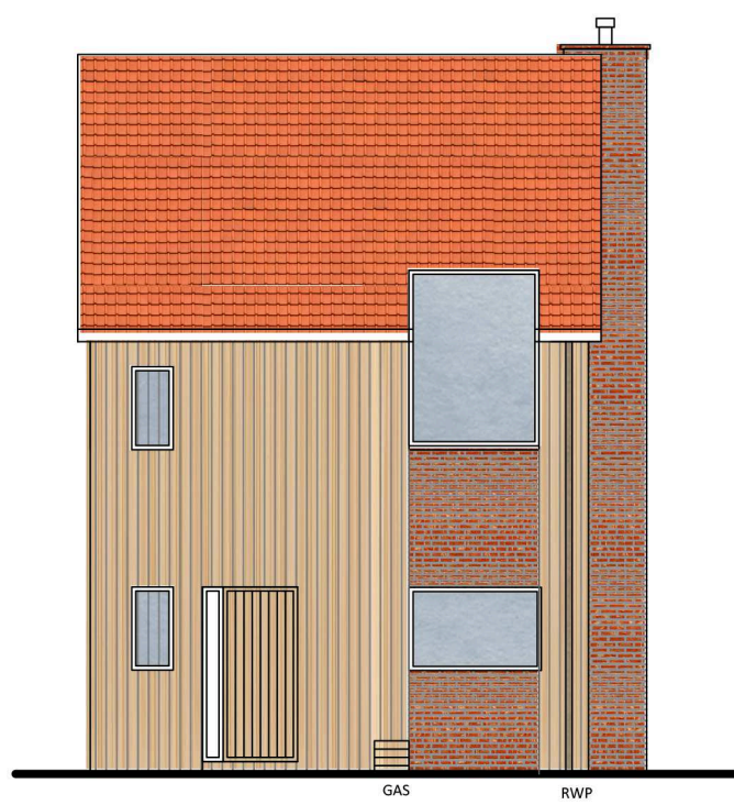
Front Elevation
