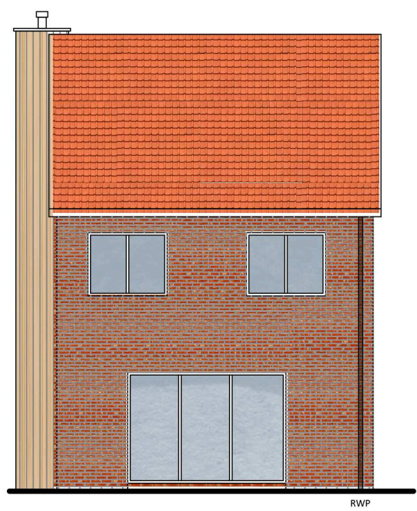
Rear Elevation
