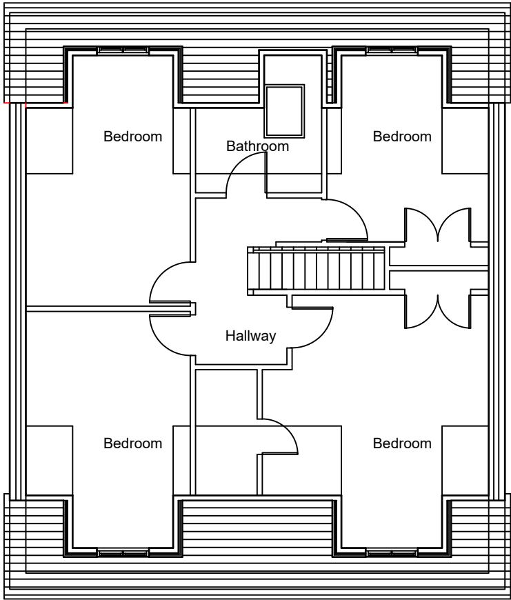
2 first floor - existing scale 1:100
