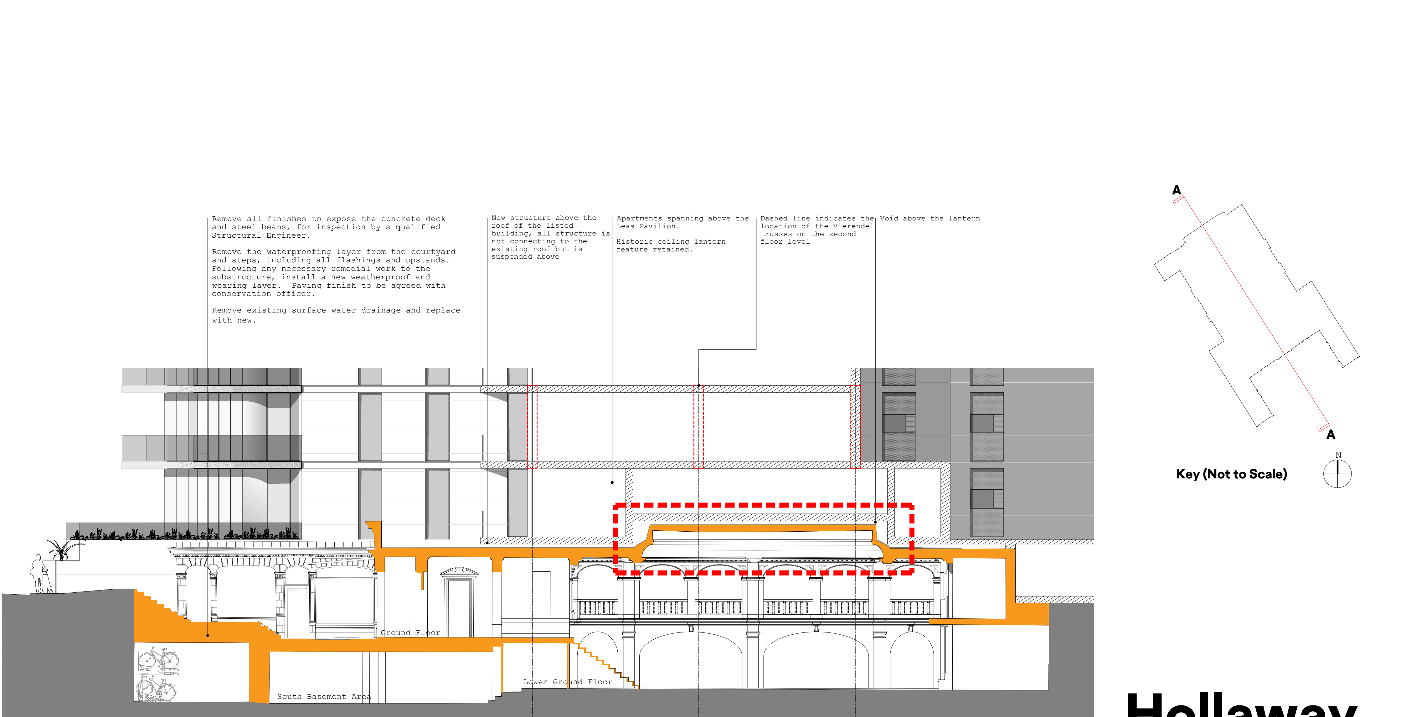
Proposed Section A-A
