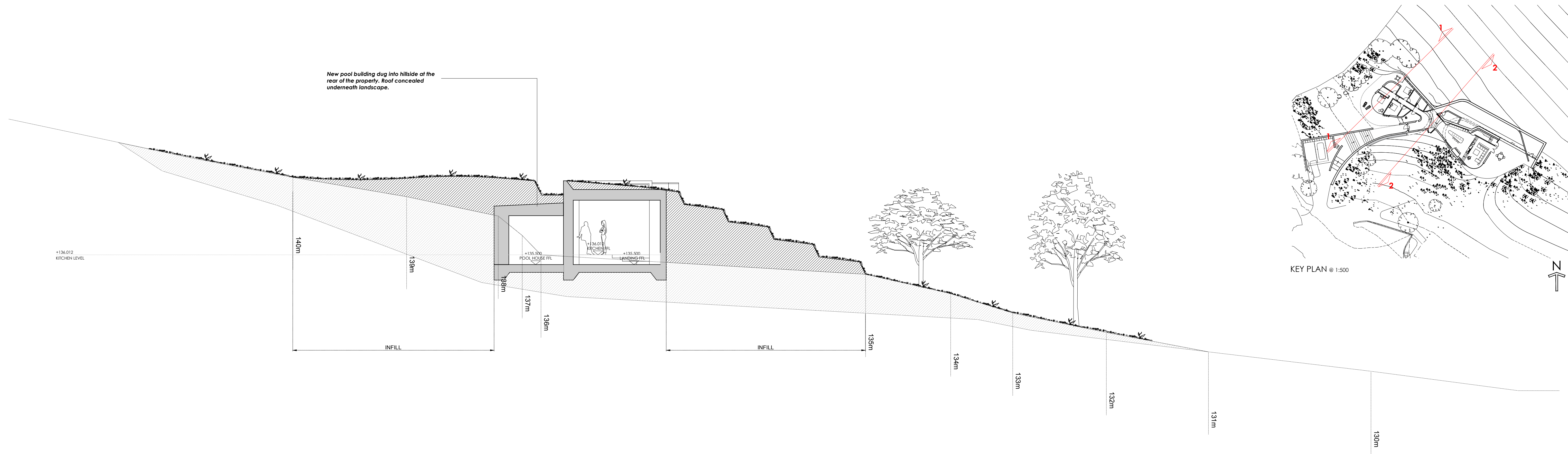
SECTION 2-2 @ 1:100
