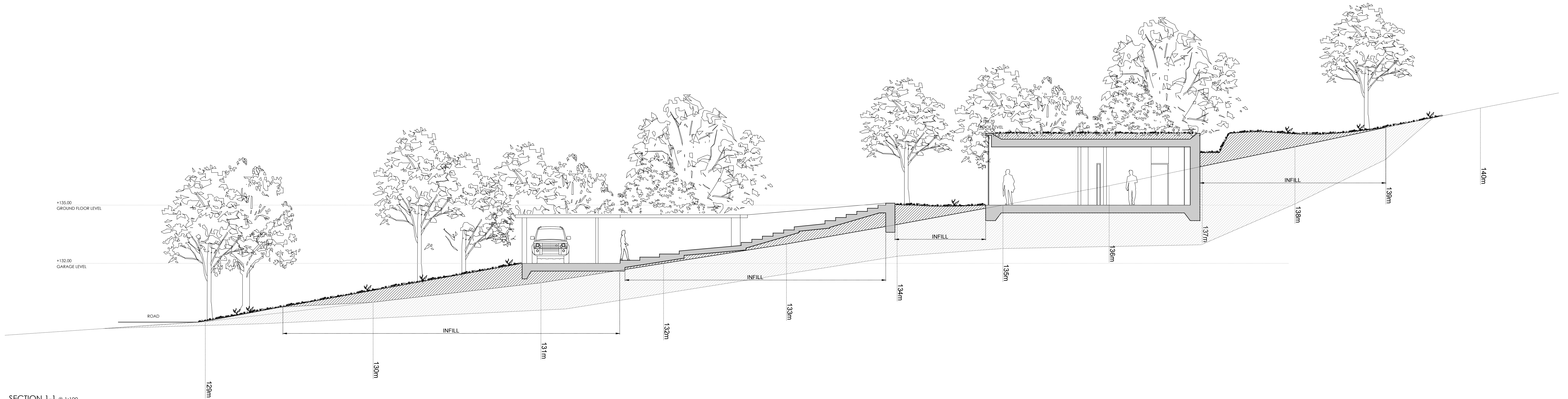
SECTION 1-1 @ 1:100
