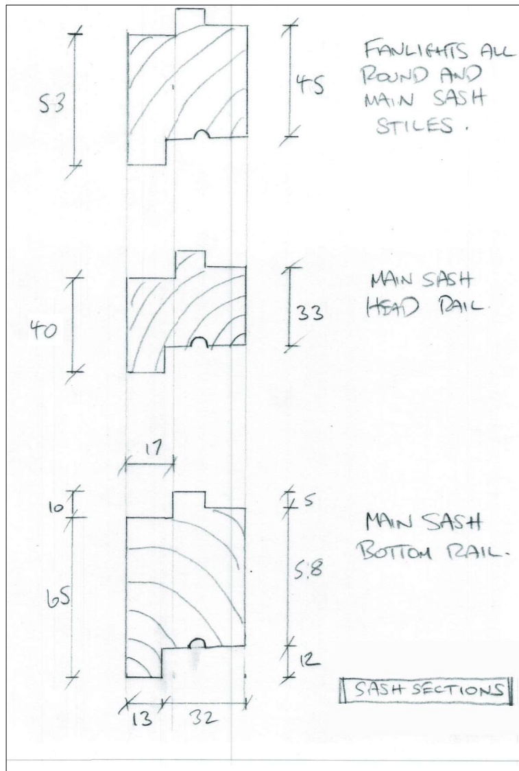
01 EXISTING VERTICAL SECTION THROUGH OPENING SASH
