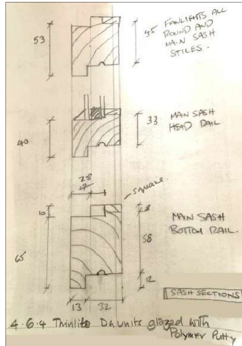
02 PROPOSED VERTICAL SECTION THROUGH OPENING SASH
