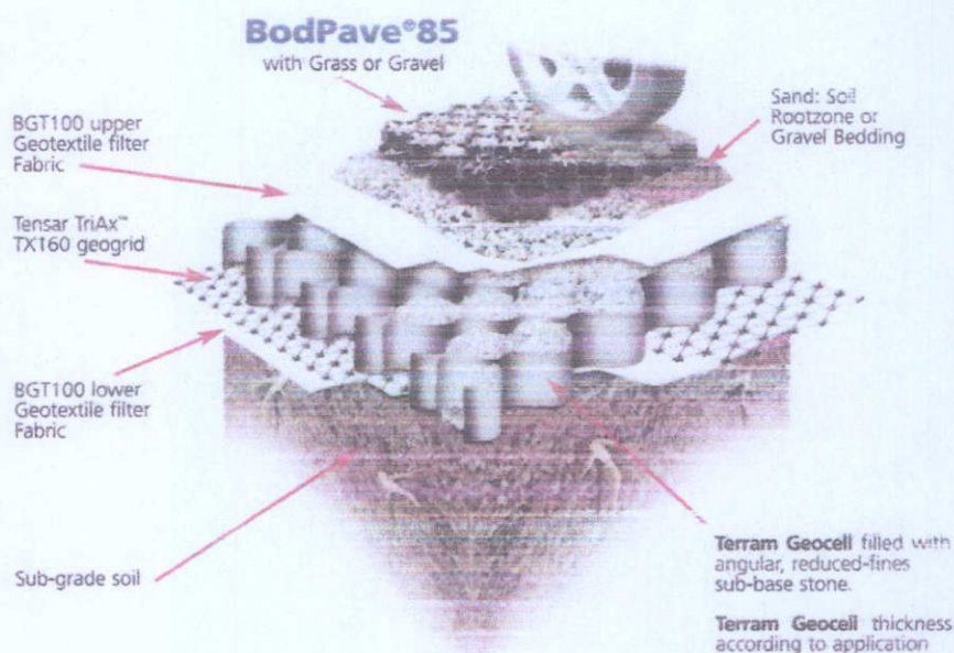
Typical Profile showing various product layers. Not all layers will apply to every application.
