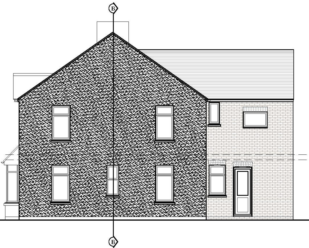
SIDE ELEVATION 1
