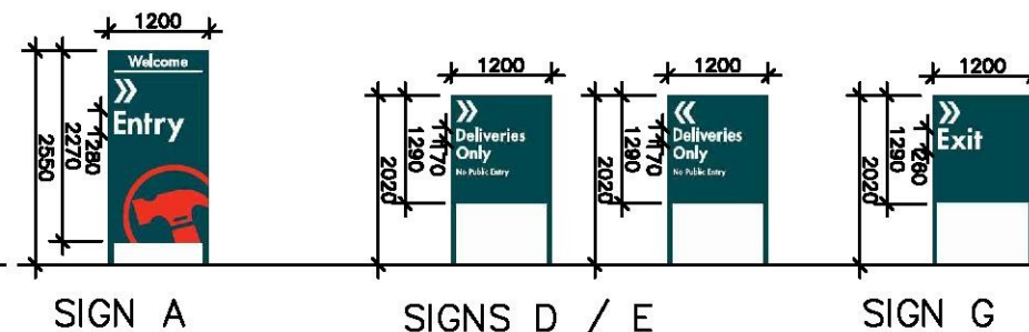
CAR PARK "PYLON" SIGNAGE 1:100
