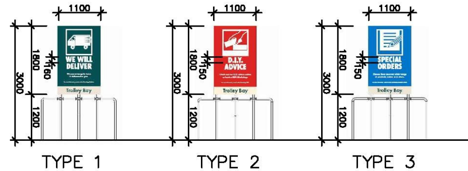
TROLLEY BAY SIGNAGE (TB) 1:100
