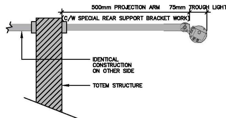
TYPICAL TROUGH LIGHT FIXING DETAIL (NOT TO SCALE)
