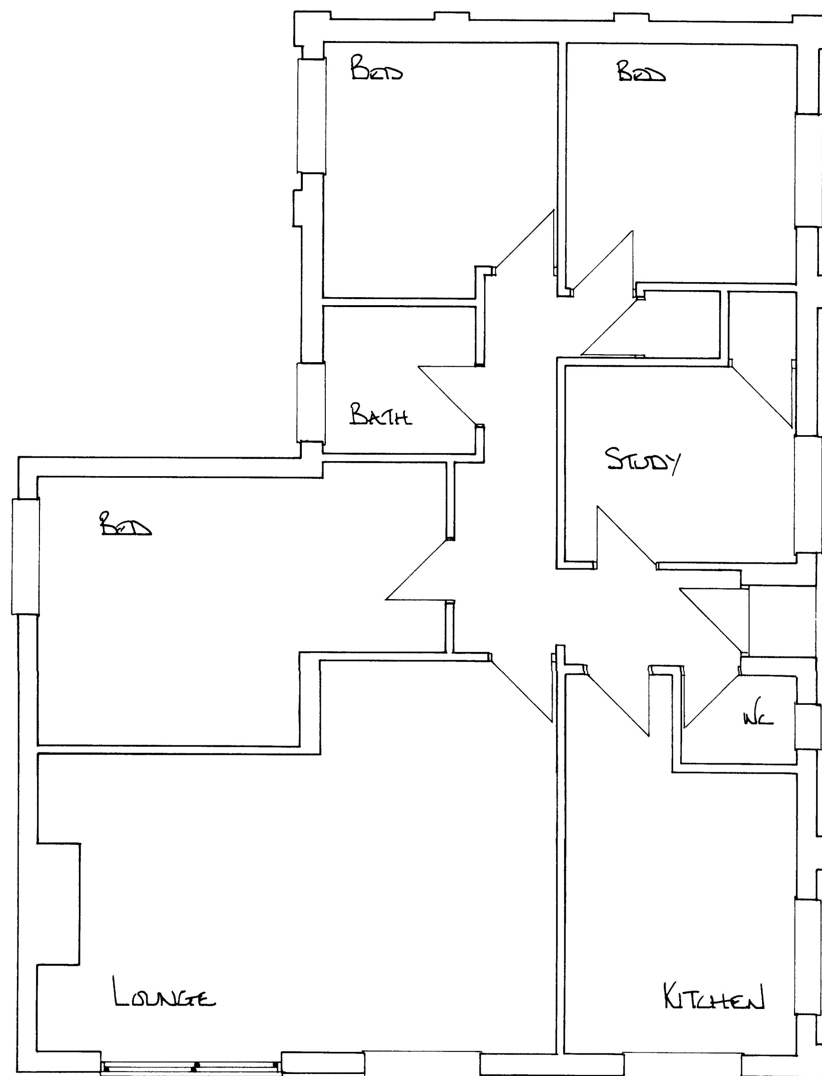
Ground floor
