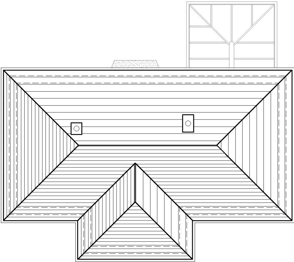
Existing Roof Plan 1:100@A3
