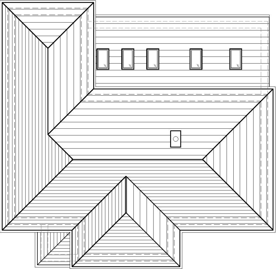
Proposed Roof Plan 1:100@A3
