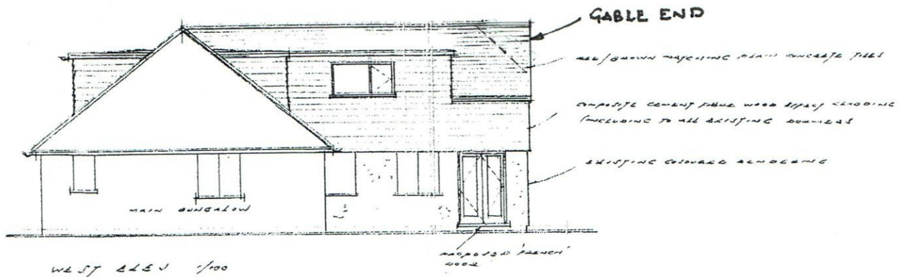
WEST ELEV 1/100
