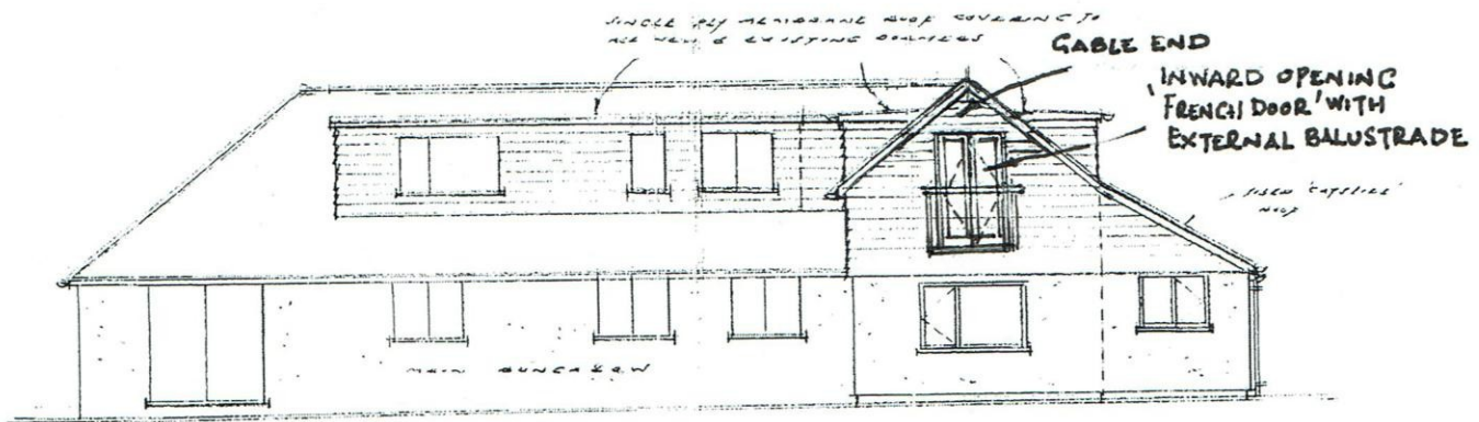
SOUTH ELEV (REAR) 1/100
