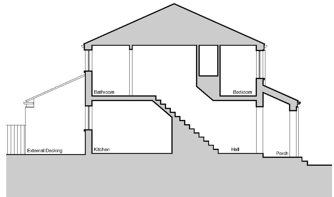
PROPOSED SECTION
