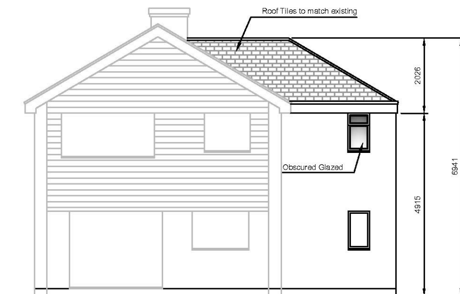
Rear Elevation
