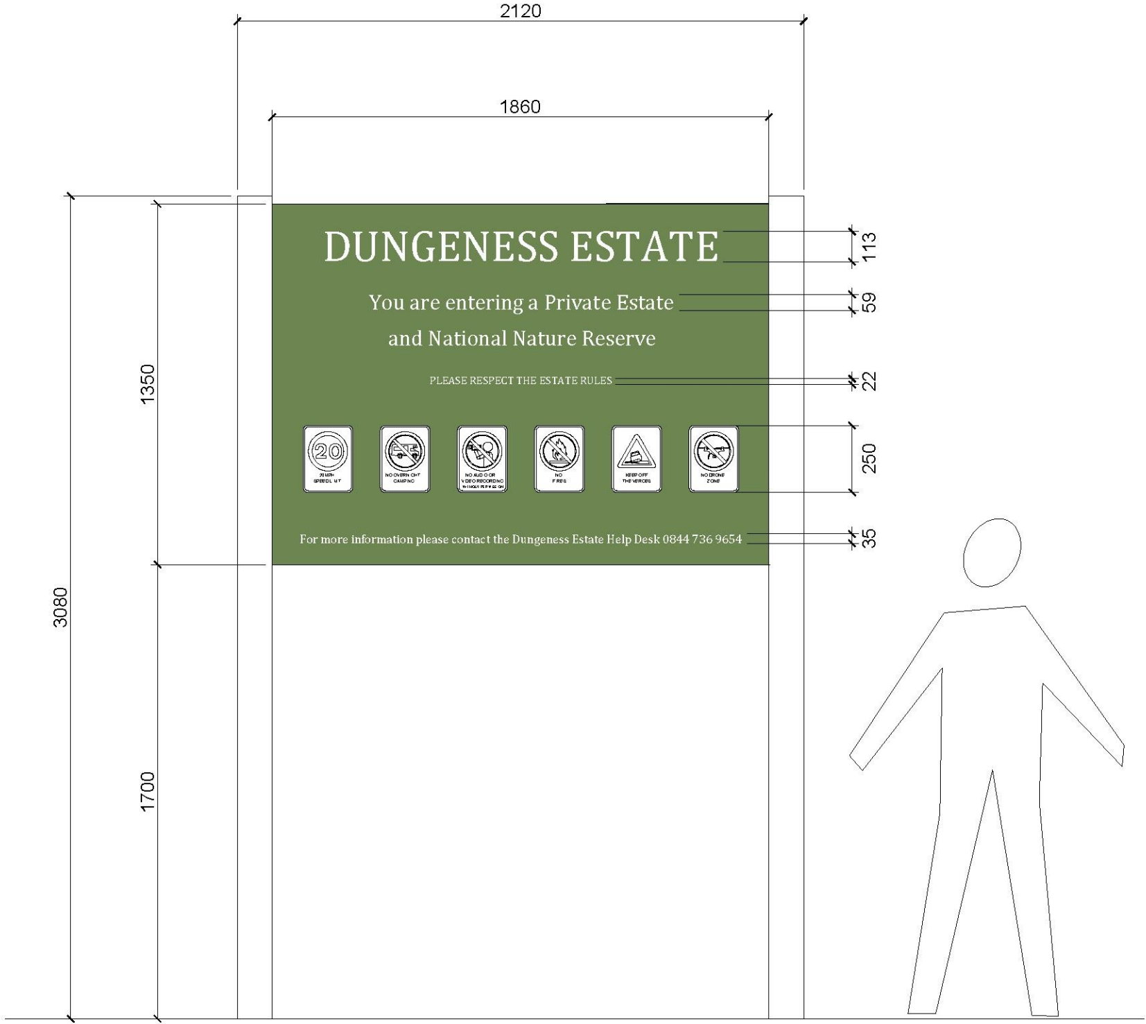
1 ELEVATION SCALE 1:10
