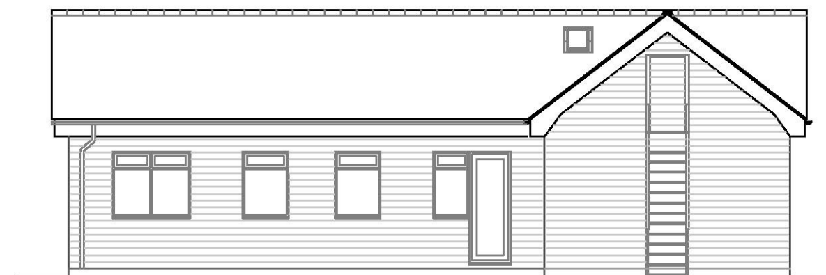
EAST ELEVATION
