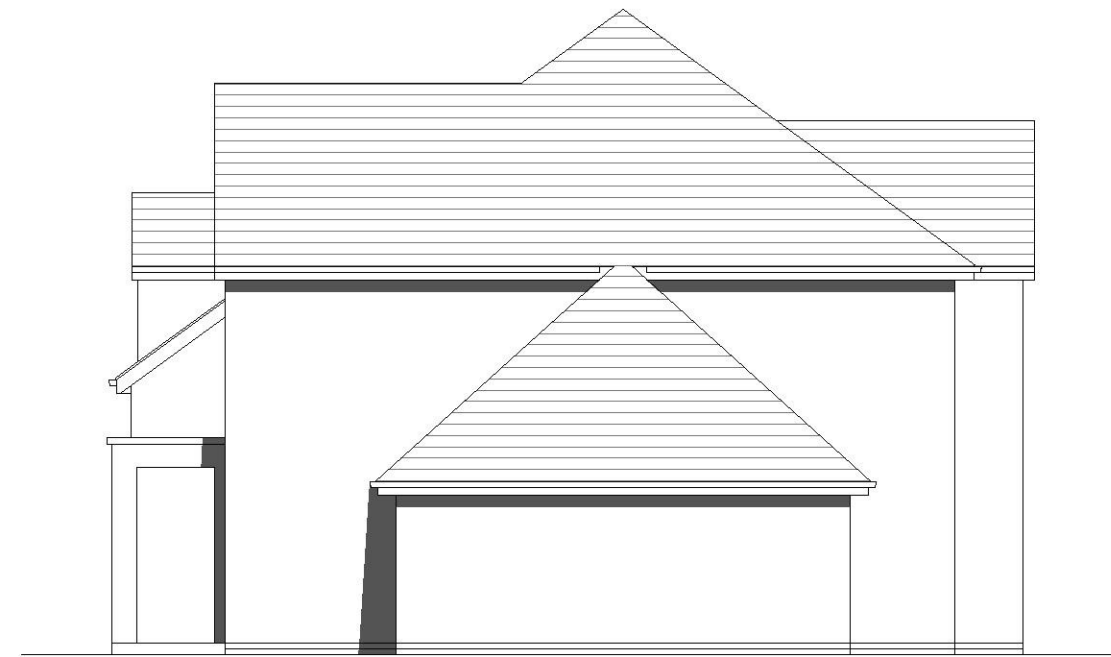
West elevation
