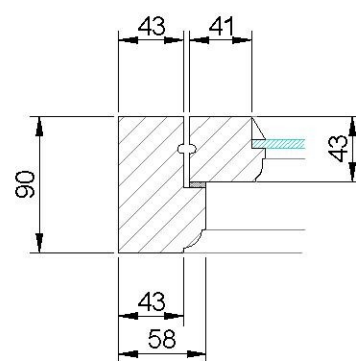
Typical Jamb Detail
