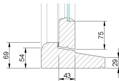
Typical Cill Detail
