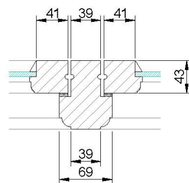
Typical Mullion Detail
