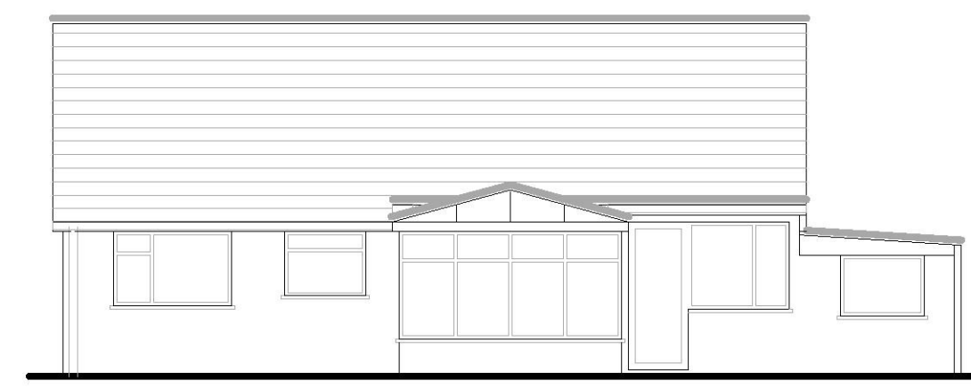
Rear Elevation Existing
