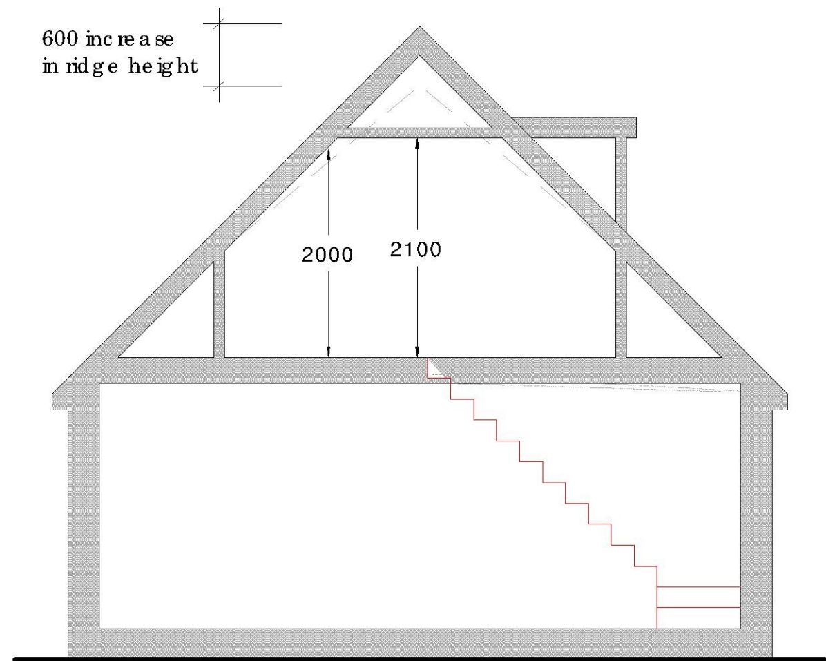
Section Proposed
