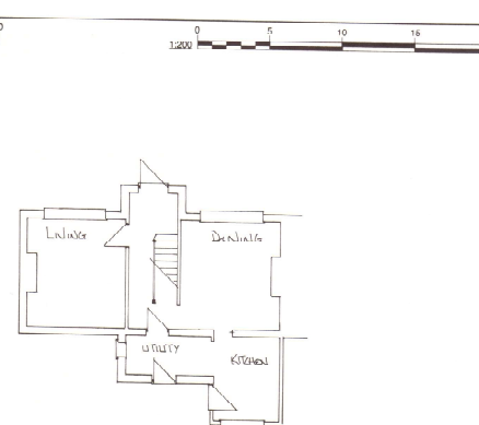
Existing layout
