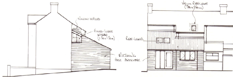
Side Proposed elevations
