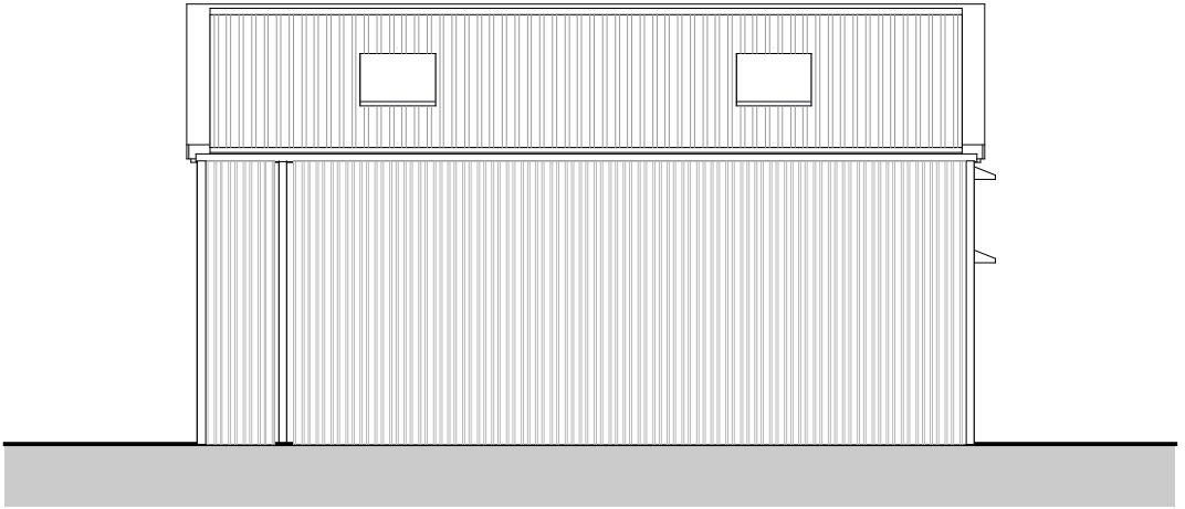
FLANK (S-E) ELEVATION
