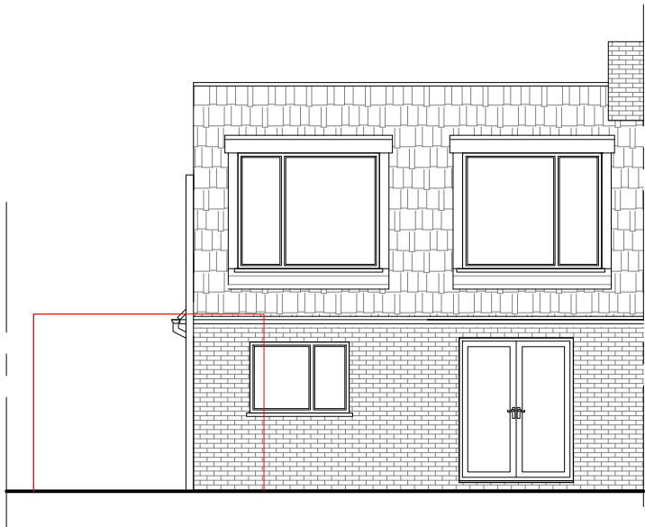
Rear Elevation
