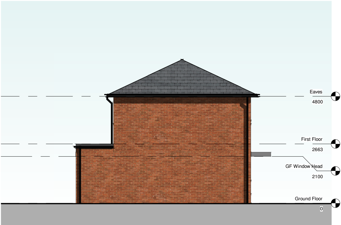
2 Side Elevation-Left 1 : 100
