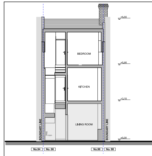
SECTION B-B
