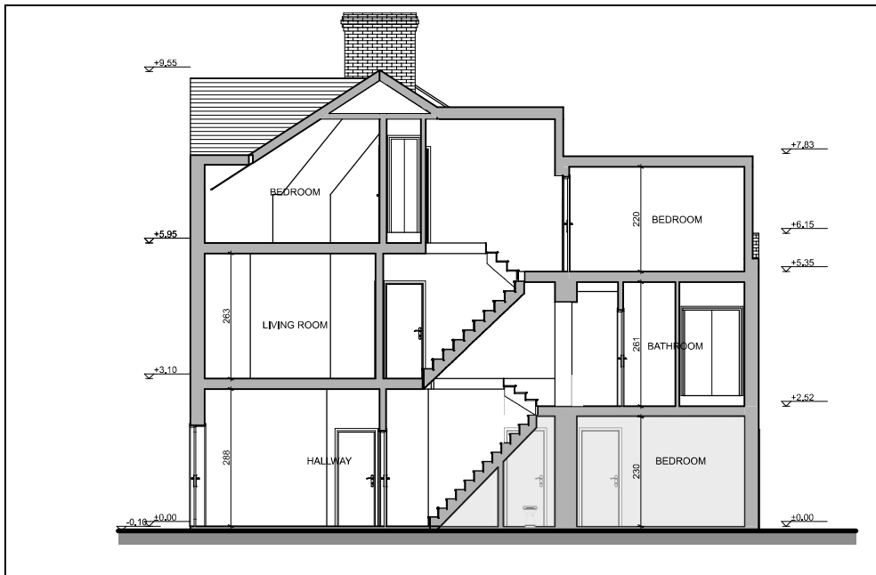
SECTION C-C
