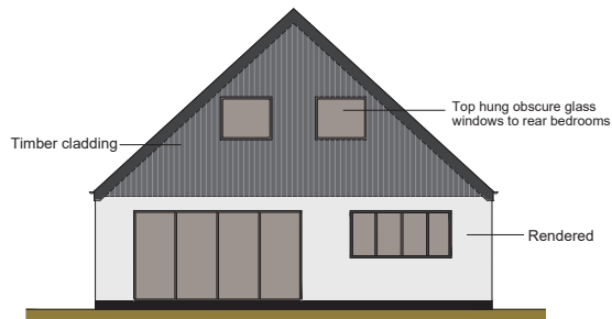
PROPOSED REAR ELEVATION (EAST)
