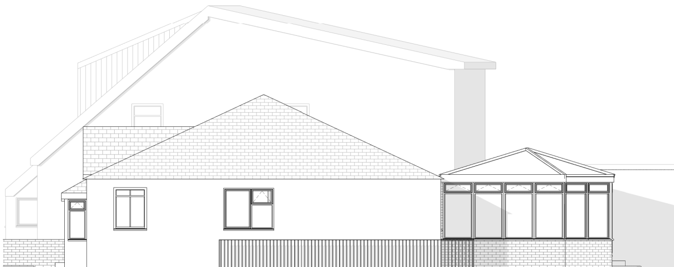
03 East Elevation 1 : 50
