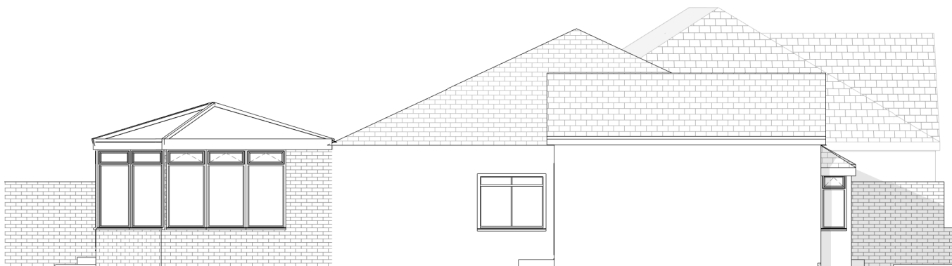
04 West Elevation 1 : 50
