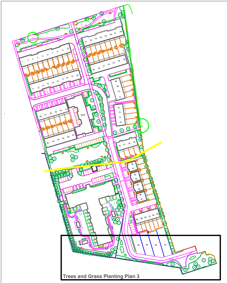
Key Plan 1:2000 @ A1
