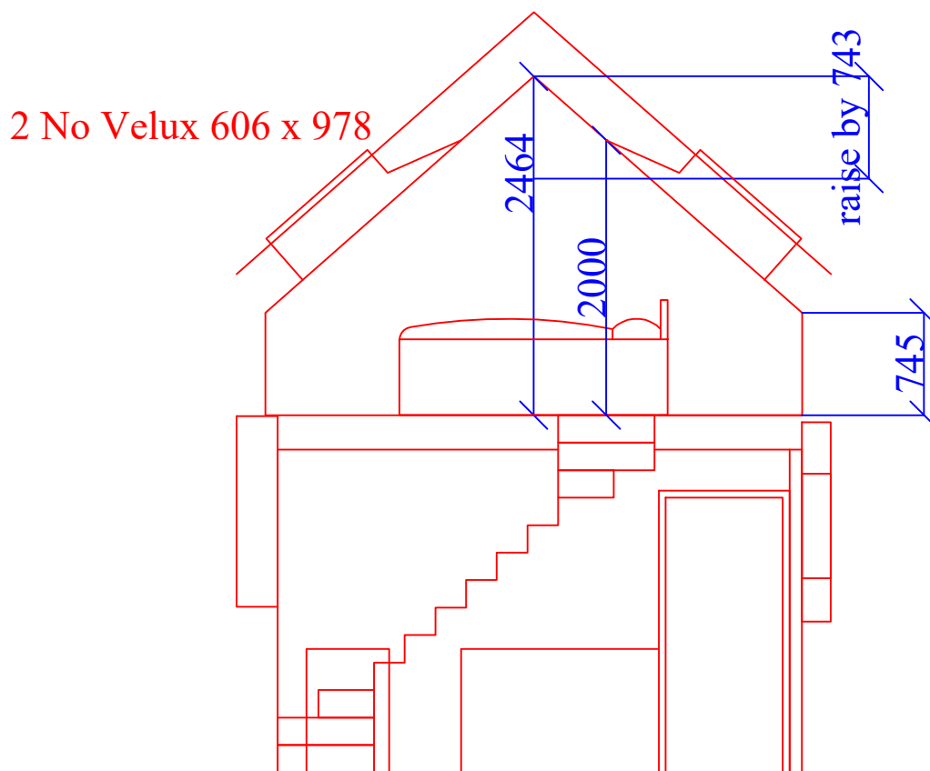
PROPOSED SECTION THROUGH 'AA'
