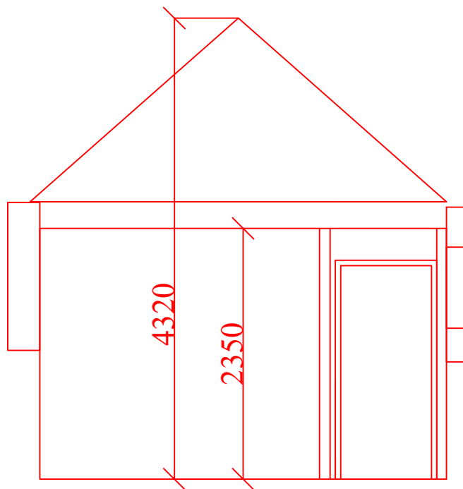
EXISTING SECTION THROUGH 'AA'
