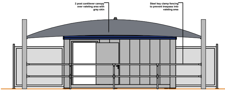
HAND CAR WASH ELEVATION VIEW B
