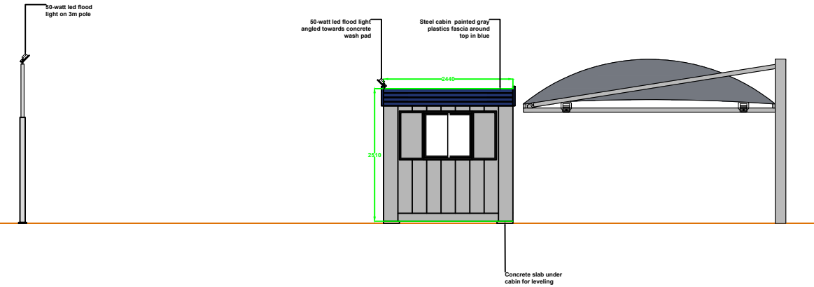
HAND CAR WASH ELEVATION VIEW C
