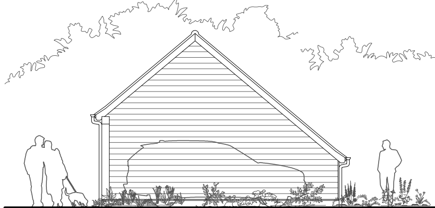
LEFT SIDE ELEVATION SCALE 1:100
