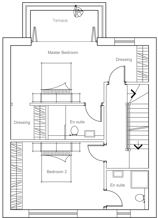
FIRST FLOOR PLAN 59.4m 2 / 639sqft
