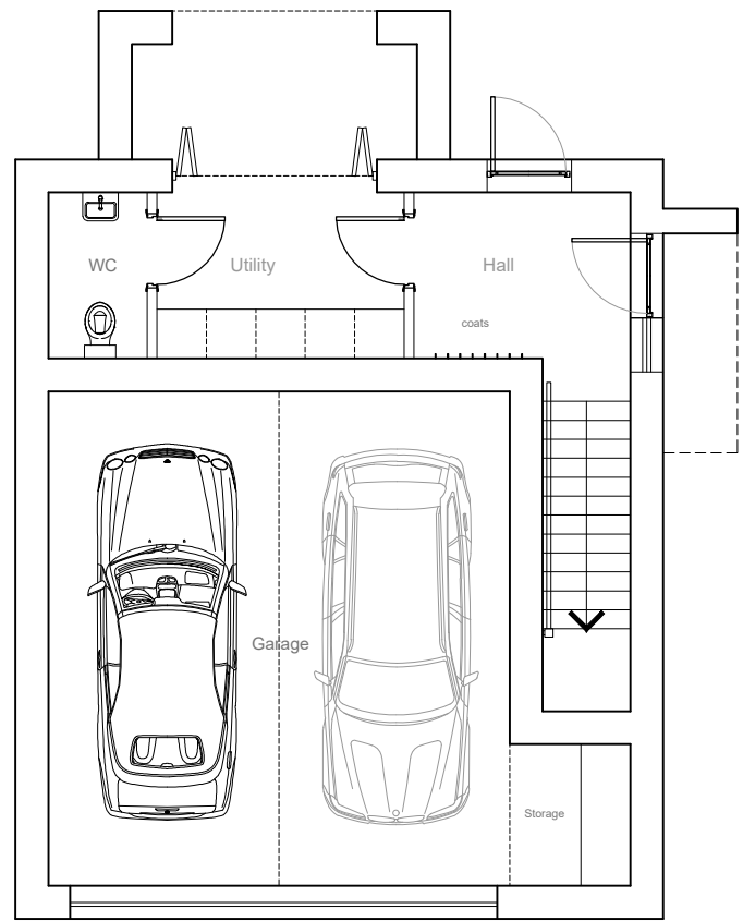
GROUND FLOOR PLAN 18.7m 2 / 201sqft
