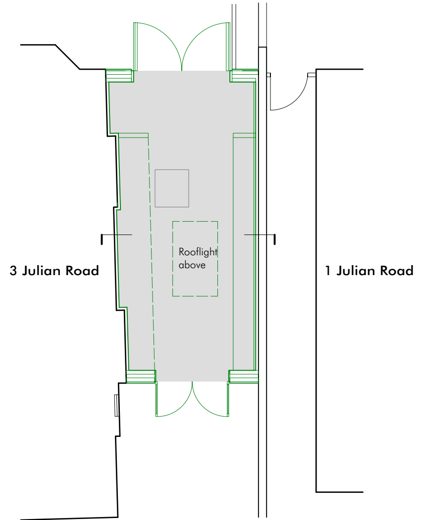
PROPOSED PLAN
