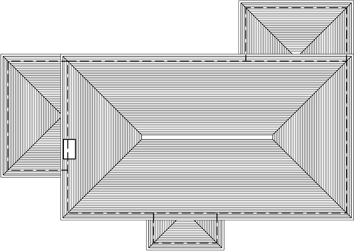
ROOF PLAN
