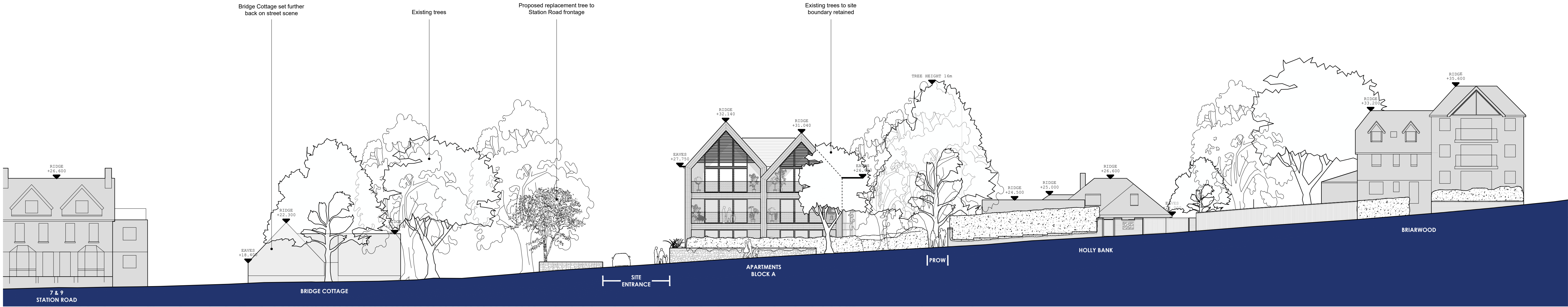
PROPOSED STREET SCENE A-A - STATION ROAD SCALE 1:200 @ A1
