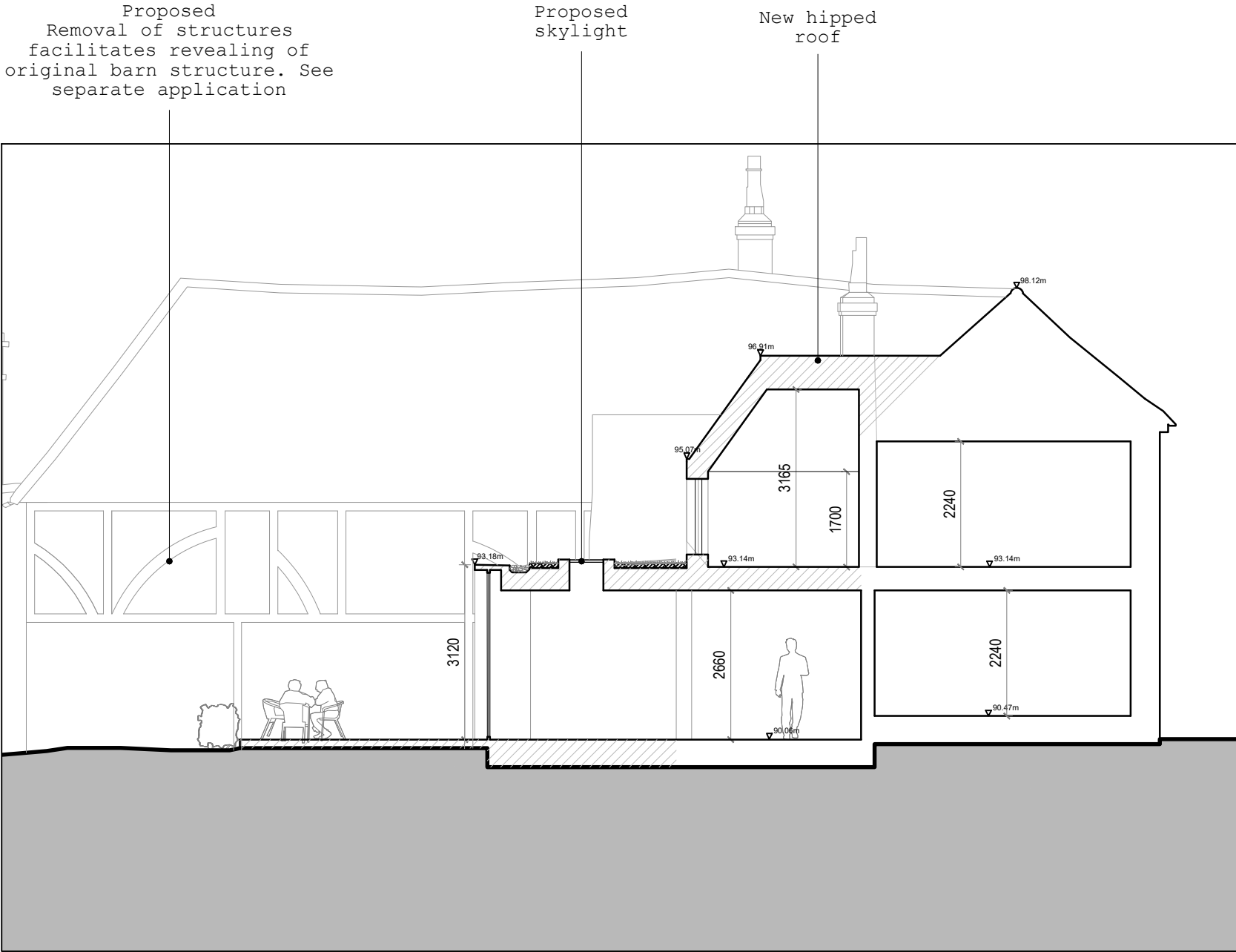
Elevation B-B @ 1:100
