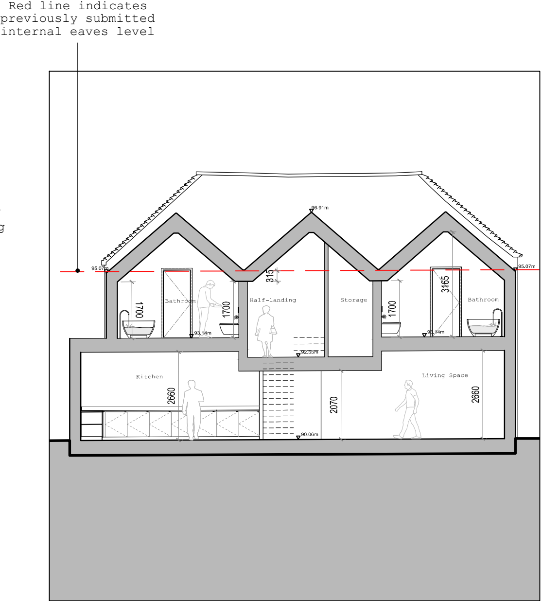
Elevation E-E @ 1:100
