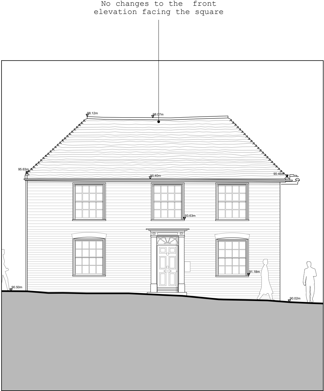
Elevation A-A @ 1:100
