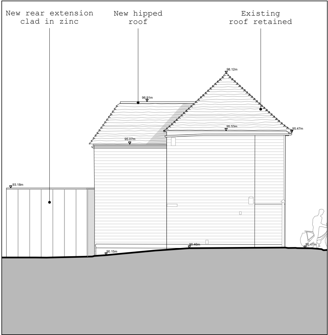
Elevation C-C @ 1:100
