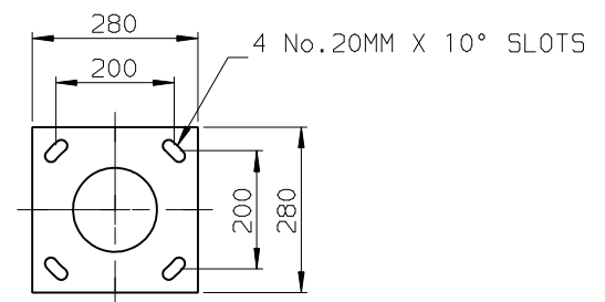
FLANGE PLATE OPTION.
