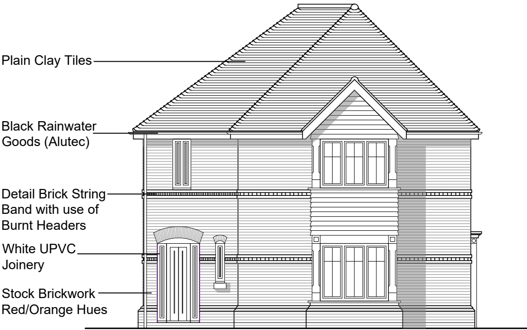
Side Elevation 1:100
