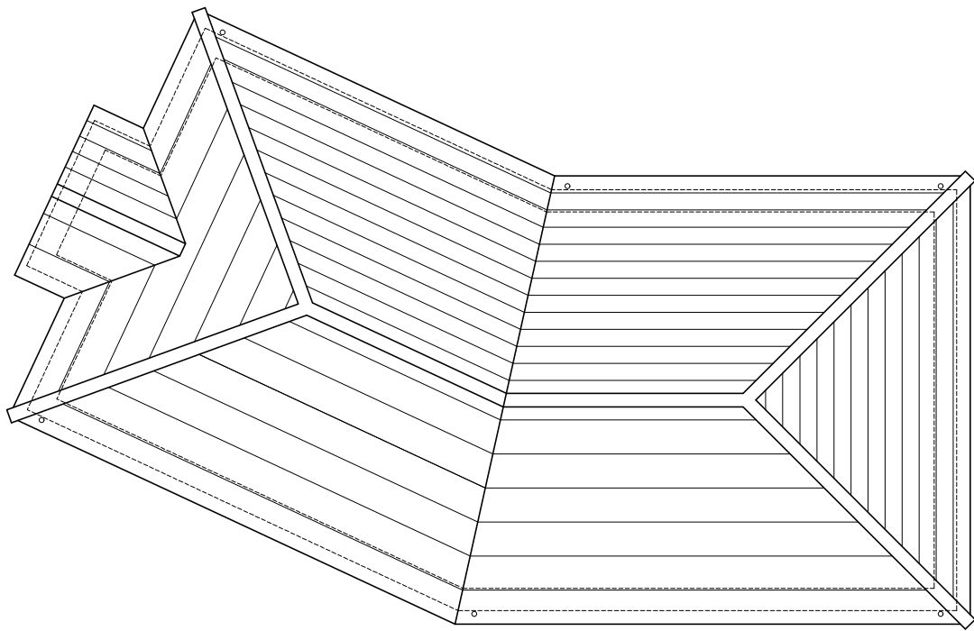
Roof Plan 1:100
