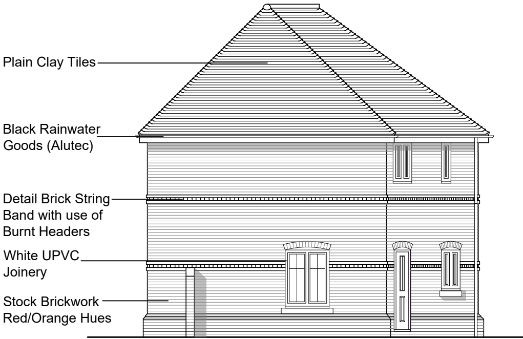
Side Elevation 1:100
