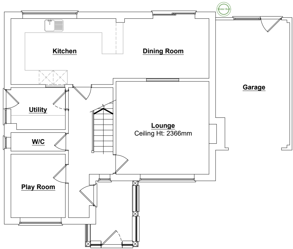
PROPOSED GROUND FLOOR LAYOUT PLAN Scale 1/100
