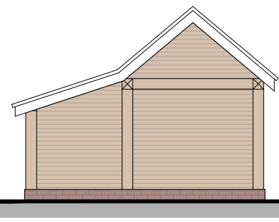
PROPOSED GARAGE ELEVATION Scale 1/100
